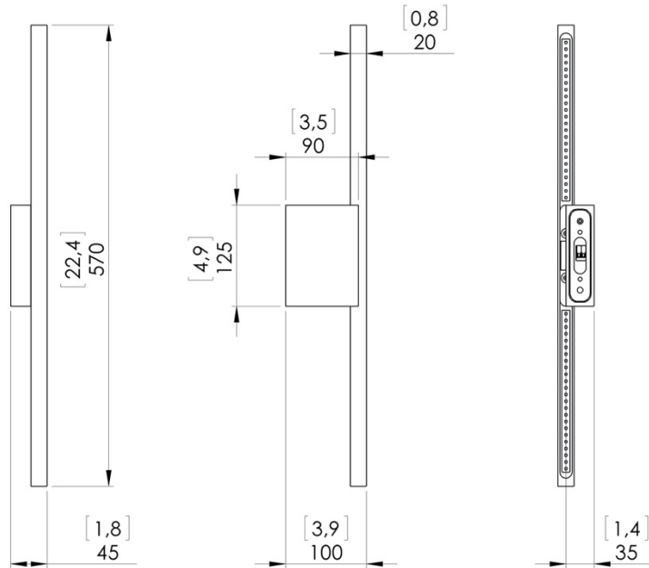
Dimensions in mm [inches]
