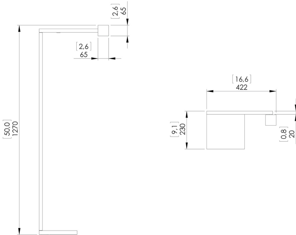
Dimensions in mm [inches]
