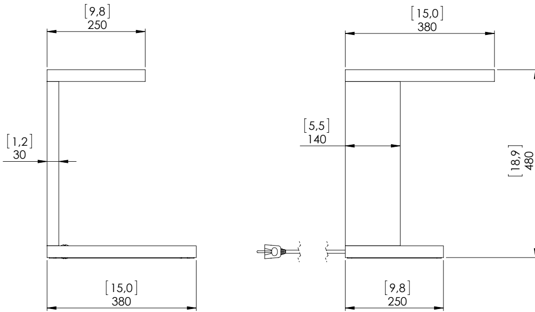
Dimensions in mm [inches]
